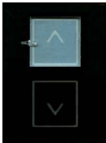
a) GlassTouch stuck with double-sided tape on glass block, b) backside of control panel, c) front side
